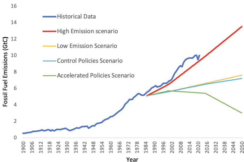
Figure 14.1: Historical emissions from 1990 until 2021 compared with the four IPCC scenarios published in 1990 for global fossil fuel emissions.
